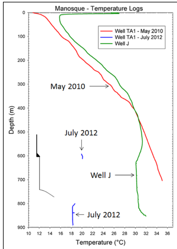
Figure 16. Temperature logs in wells TA1 and J.
